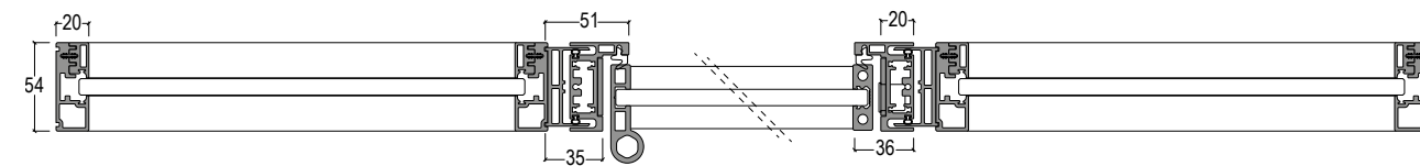
Stipite Cube abbinato a porta a battente 180 e vetrate fisse _Cube frame combined with Hinged door 180 and fixed glass panels
