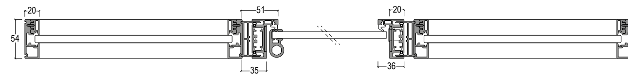
Stipite Cube abbinato a porta a battente Vitra e vetrate fisse _Cube frame combined with Vitra Hinged door and fixed glass panels
